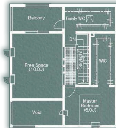
2F Plan
